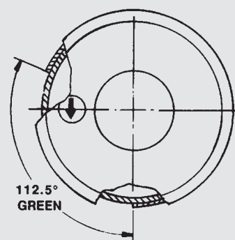
BASE MOUNT STARBOARD SIDE LIGHT
