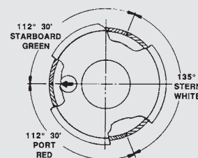
0200 SERIES ONLY BASE MOUNT TRI-COLOR LIGHT
