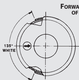
BASE MOUNT STERN LIGHT
